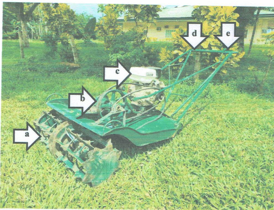
Figure 1. Parts of the HG AIM HG-TUT-YD16 Walking-Type Agricultural Tractor powered by an 11.94 kW YAMADA Gasoline Engine include the following: (a) Tilling wheel, (b) V-belt and pulley transmission system, (c) Prime mover, (d) Handle, and (e) Main clutch lever.
